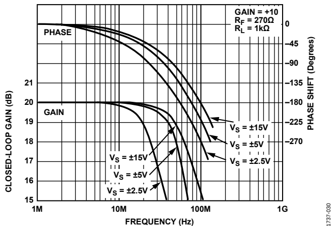
Figure 32. Closed-Loop Gain and Phase Shift vs. Frequency, G = +10 , R_L = 1\text{ k}\Omega
