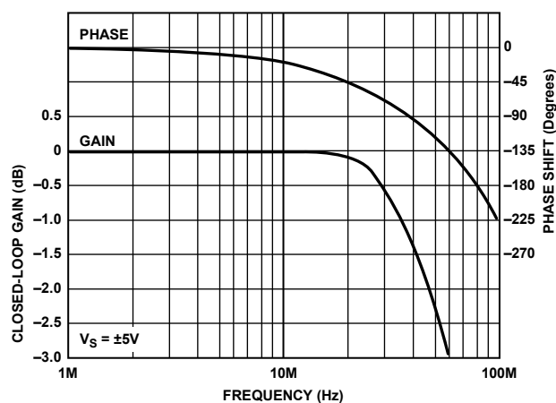
Figure 60. Closed-Loop Gain and Phase Shift vs. Frequency for 2:1 Mux, On Channel
